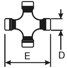
U-Joint
